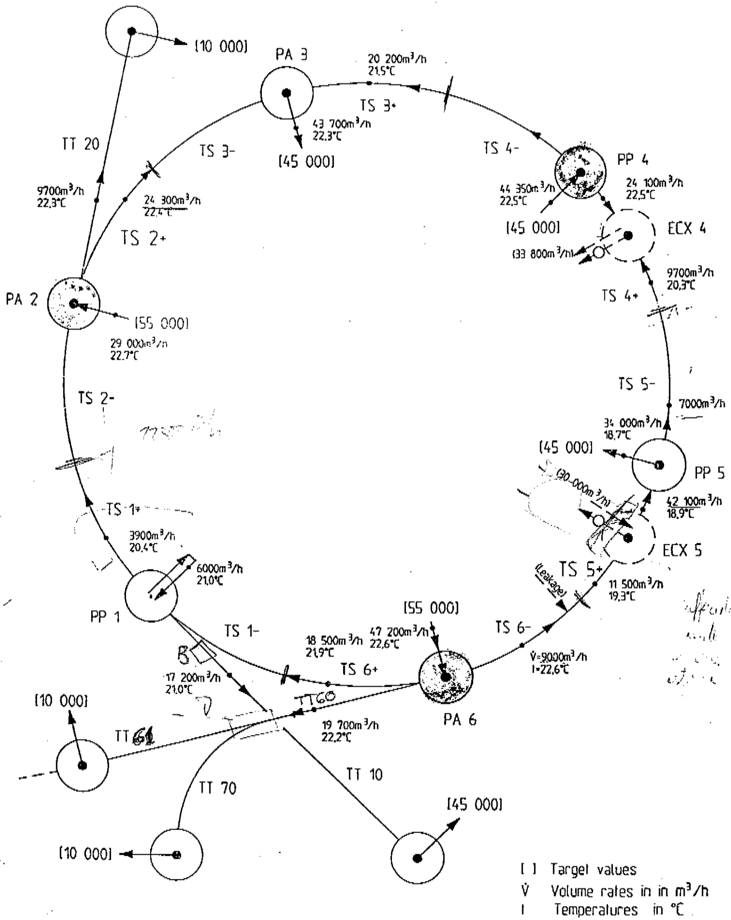
Figure 5 Distribution of air flow rates and temperatures in the tunnel
